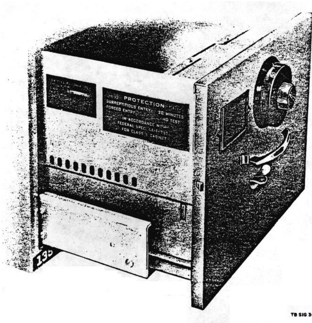
Figure 3. Single drawer security file showing Federal Specification AA-F-358b label.
